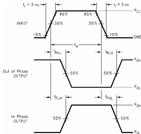
FIGURE 3. AC Waveforms
