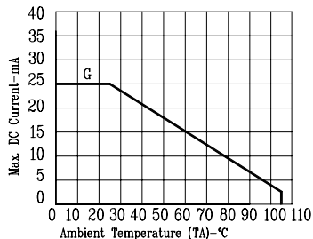
Fig5. MAX. ALLOWABLE DC CURRENT VS. AMBIENT TEMPERATURE.
