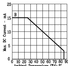
Fig5. MAX. ALLOWABLE DC CURRENT VS. AMBIENT TEMPERATURE.
