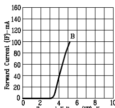
Fig3. FORWARD CURRENT VS. FORWARD VOLTAGE
