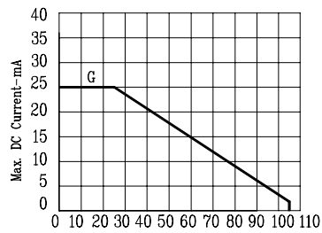
Fig5. MAX. ALLOWABLE DC CURRENT VS. AMBIENT TEMPERATURE.
