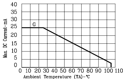
Fig5. MAX. ALLOWABLE DC CURRENT VS. AMBIENT TEMPERATURE.
