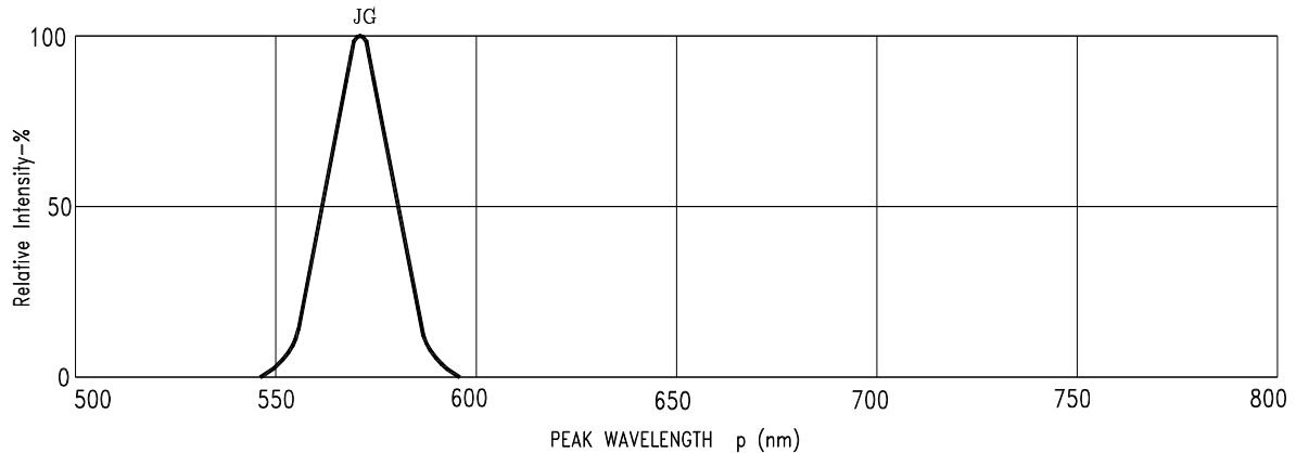
Fig1. Spectral Emission
