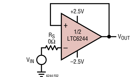
Figure 2. Unity Gain Follower Test Circuit
