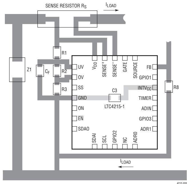
Figure 5. Recommended Layout
