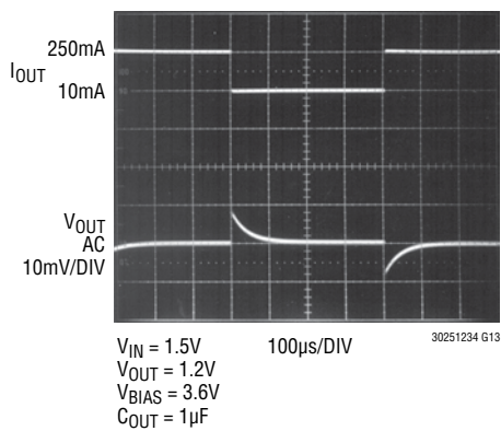
Transient Response
