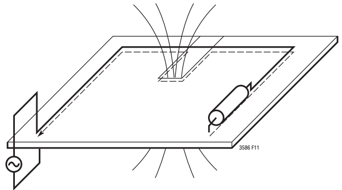
Figure 11. Higher Frequency Ground Currents Follow Their Incident Path. Slits in the Ground Plane Cause High Voltage and Increased Emissions
