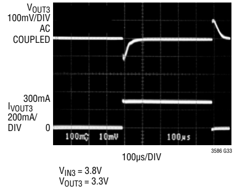
Buck-Boost Step Response
