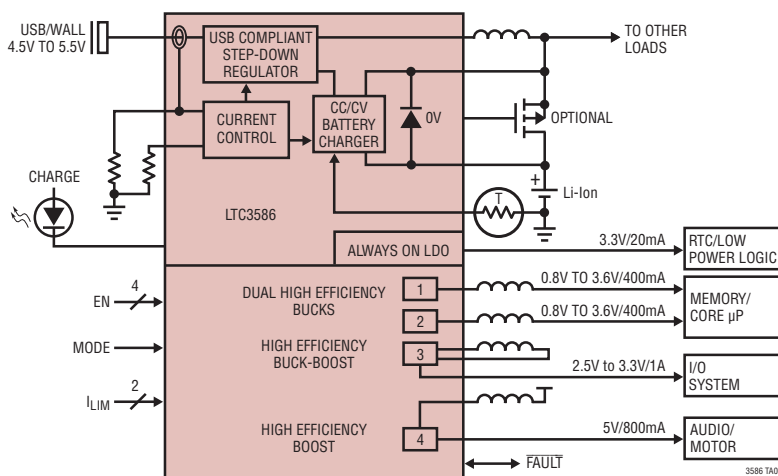
High Efficiency PowerPath Manager, Dual Buck, Buck-Boost and Boost
