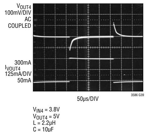
Boost Step Response (50mA to 300mA)
