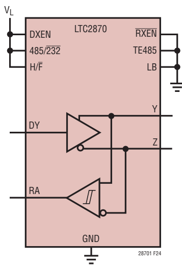
Figure 24. LTC2870 in RS485 Mode Half-Duplex
