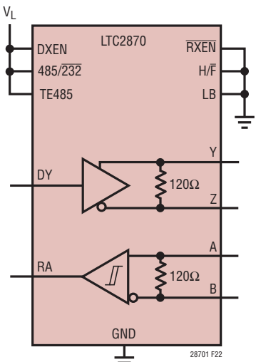
Figure 22. LTC2870 in RS485 Mode, Terminated
