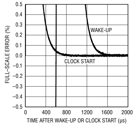
LTC2216/LTC2215 Full-Scale Settling After Wake-Up from Shutdown or Starting Encode Clock
