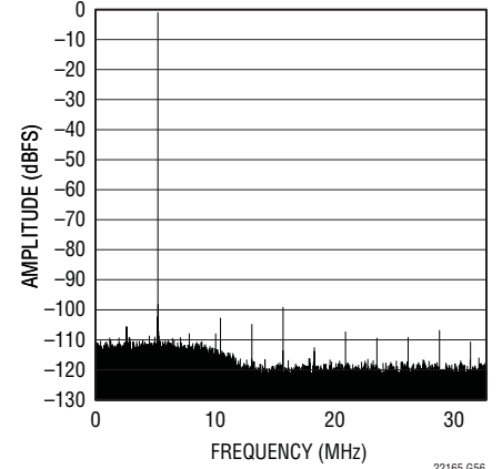
LTC2215 64k Point FFT, f_{IN} = 70.2\text{MHz} , -1\text{dBFS}
