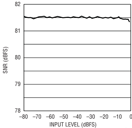
LTC2215 SNR vs Input Level, f_{IN} = 15.2\text{MHz}
