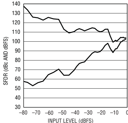
LTC2215 SFDR vs Input Level, f_{IN} = 15.2\text{MHz} , Dither "Off"
