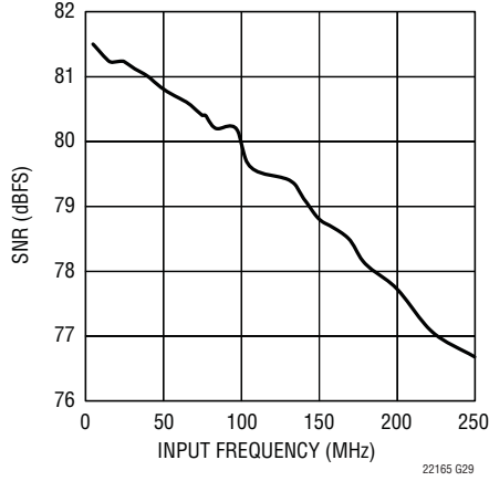
LTC2216 SNR vs Input Frequency
