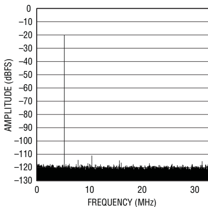
LTC2215 64k Point FFT, f_{IN} = 70.1\text{MHz} , -20\text{dBFS} , Dither "Off"
