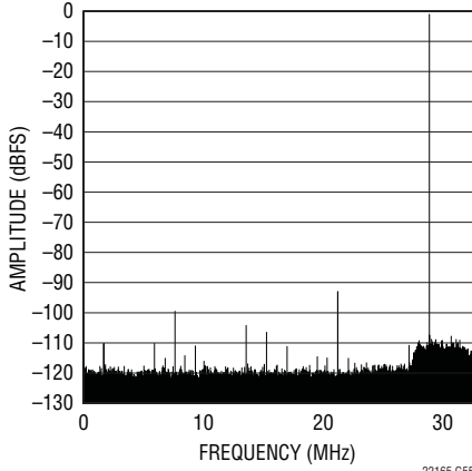
LTC2215 64k Point FFT, f_{IN} = 28.7\text{MHz} , -1\text{dBFS}
