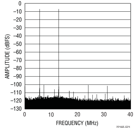
LTC2216 64k Point 2-Tone FFT, f_{IN} = 67.2\text{MHz} and 74.4\text{MHz} , -7dBFS
