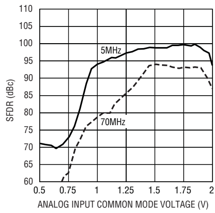
LTC2216 SFDR vs Analog Input Common Mode Voltage, 5MHz and 70MHz, -1\text{dBFS}
