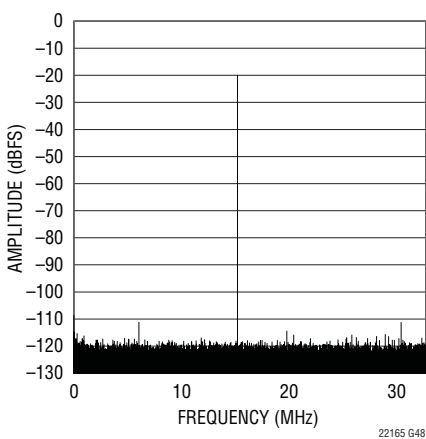
LTC2215 64k Point FFT, f_{IN} = 15.1\text{MHz} , -20\text{dBFS} , Dither "Off"
