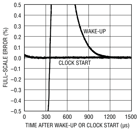
LTC2216/LTC2215 Mid-Scale Settling After Wake-Up from Shutdown or Starting Encode Clock
