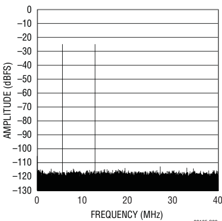
LTC2216 64k Point 2-Tone FFT, f_{IN} = 67.2\text{MHz} and 74.4\text{MHz} , -25dBFS, Dither "On"
