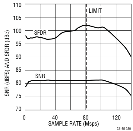
LTC2216 SNR and SFDR vs Sample Rate, f_{IN} = 5.2\text{MHz}
