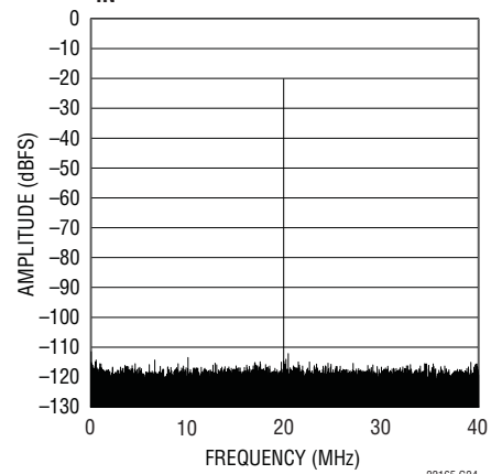
LTC2216 64k Point FFT, f_{IN} = 140.1\text{MHz} , -20dBFS, Dither "On"
