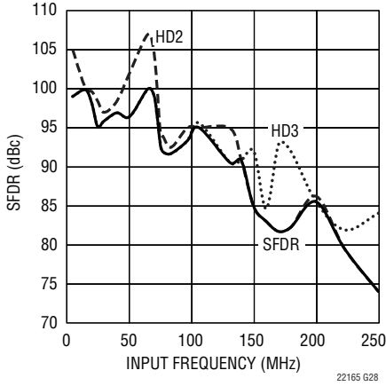
LTC2216 SFDR (HD2 and HD3) vs Input Frequency
