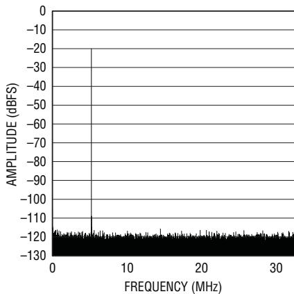
LTC2215 64k Point FFT, f_{IN} = 70.1\text{MHz} , -20\text{dBFS} , Dither "On"
