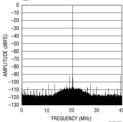
LTC2216 64k Point FFT, f_{IN} = 140.5\text{MHz} , -1dBFS
