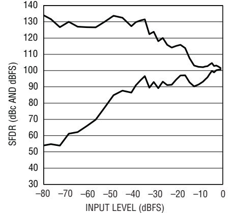
LTC2215 SFDR vs Input Level, f_{IN} = 15.2\text{MHz} , Dither "On"
