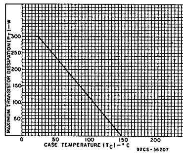
Fig. 5 - Power derating curve for all types.
