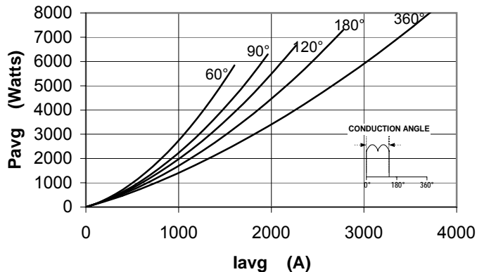
Maximum On-State Power Dissipation Square Waveform
