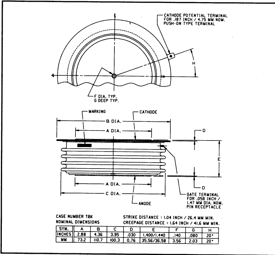
TBK7 3000A Phase Control SCR 3000 Amperes Average, 600 Volts
