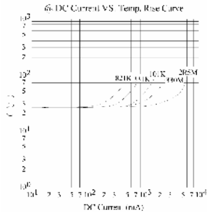
DC Current VS. Temp. Rise Curve
