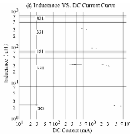
Inductance VS. DC Current Curve
