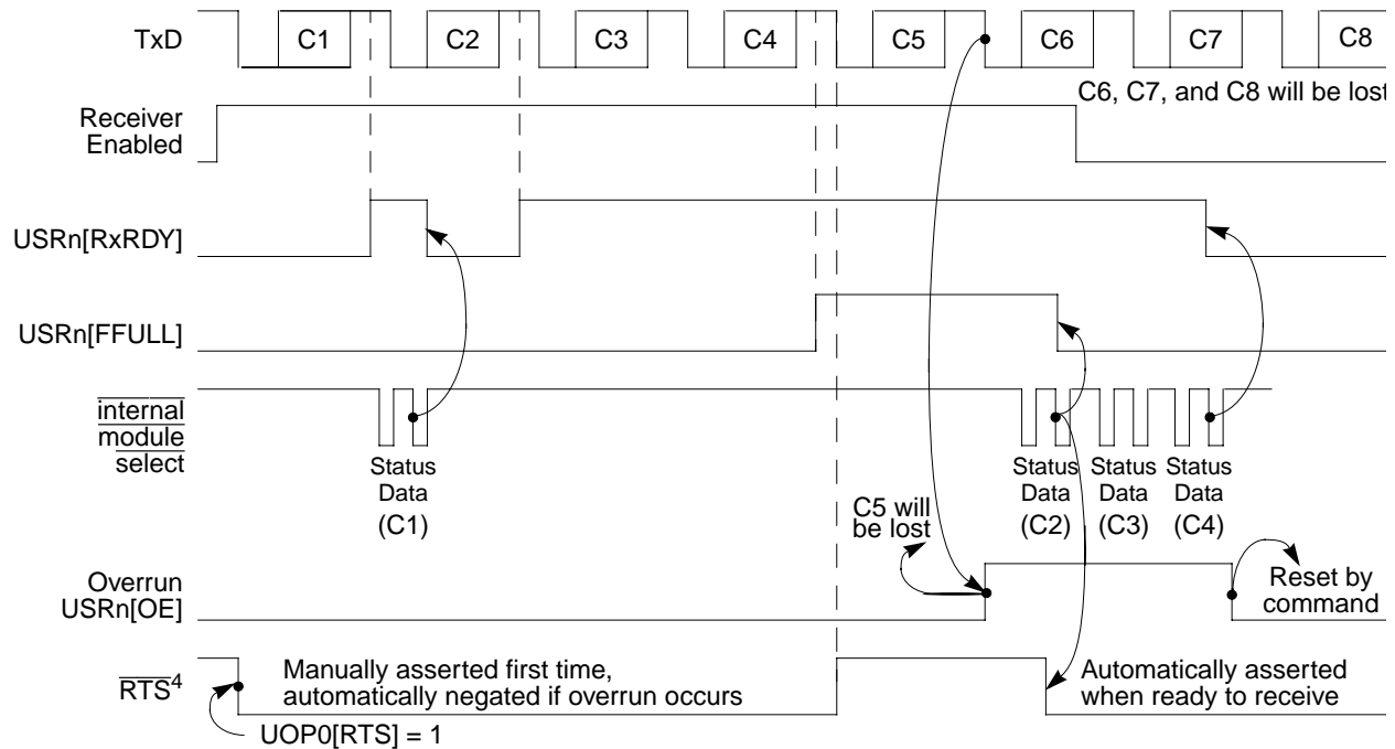
Figure 14-22. Receiver Timing
