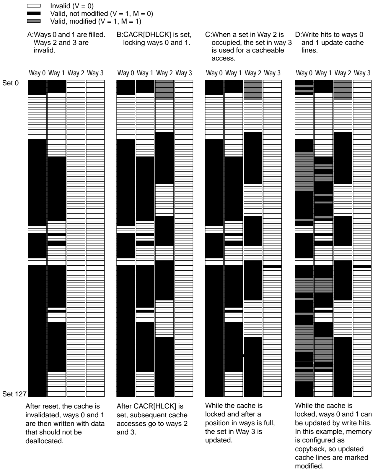
Figure 4-7. Cache Locking
