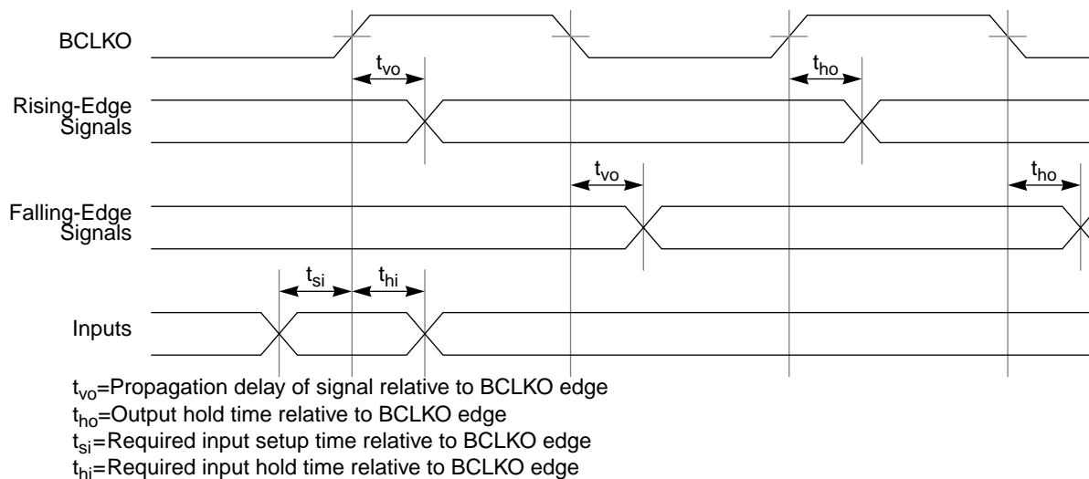
Figure 18-1. Signal Relationship to BCLKO for Non-DRAM Access
