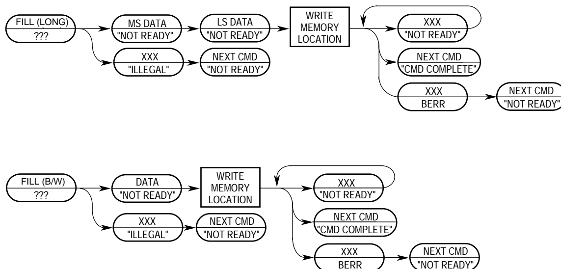
Figure 5-29. FILL Command Sequence
