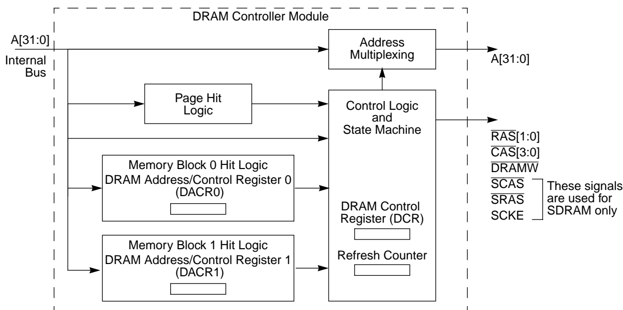
Figure 11-1. Asynchronous/Synchronous DRAM Controller Block Diagram
