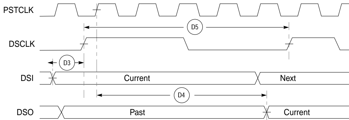
Figure 20-13. BDM Serial Port AC Timing
