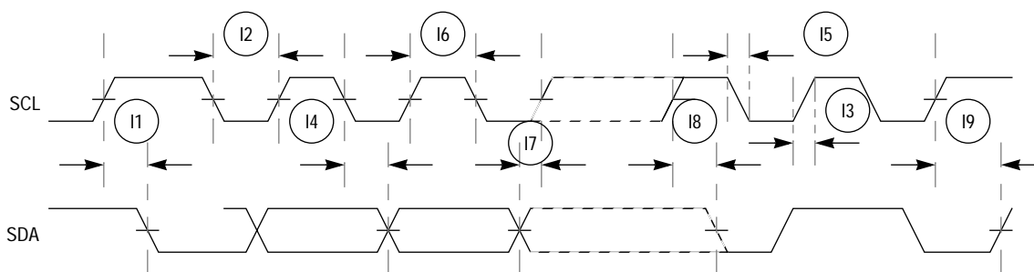
Figure 20-15. I 2 C Input/Output Timings
