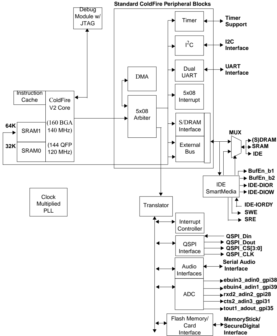
Figure 1. MCF5249 Block Diagram
