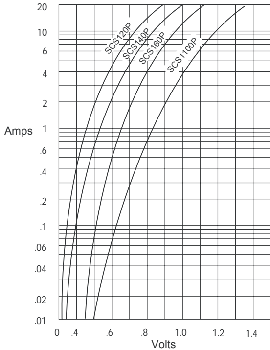
FIG.1 TYPICAL FORWARD CHARACTERISTICS
