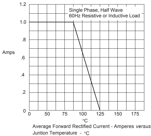
FIG.3-FORWARD DERATING CURVE
