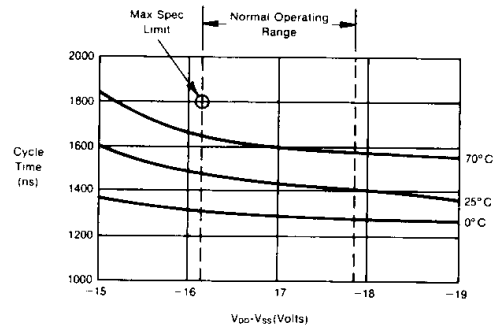
Fig.4 TYPICAL CYCLE TIME vs. POWER SUPPLY VOLTAGE
