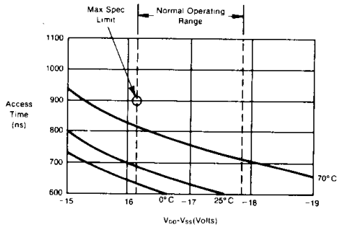
Fig.3 TYPICAL ACCESS TIME vs. POWER SUPPLY VOLTAGE
