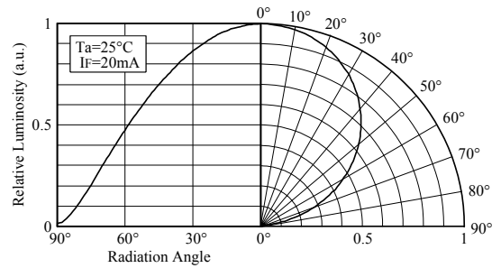
■ Directivity (NSCR426B)
