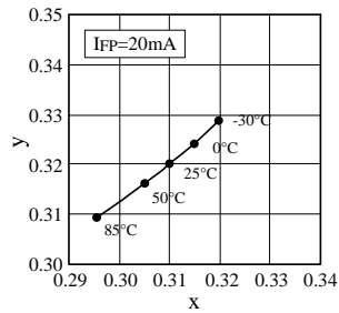
■ Ambient Temperature vs. Chromaticity Coordinate
