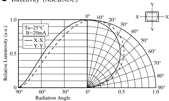
■ Directivity (NSCB505C)
