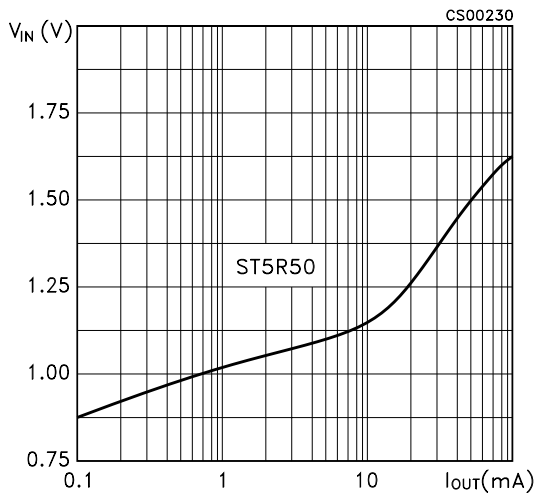
Figure 25: Minimum Input Voltage vs Output Current
