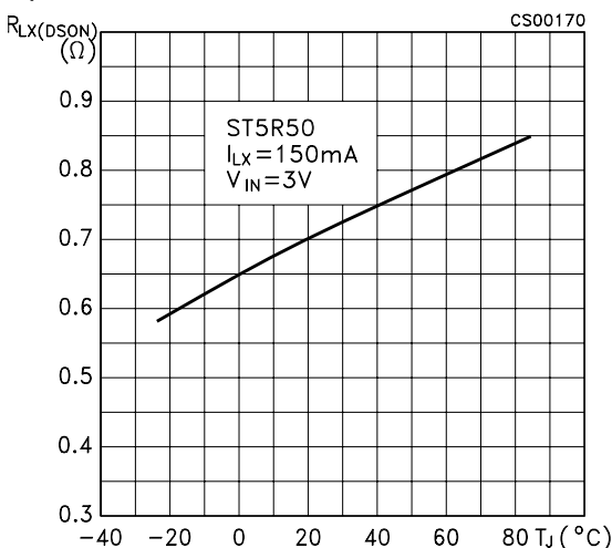
Figure 26: Internal Switch R_{DSON} vs Temperature
