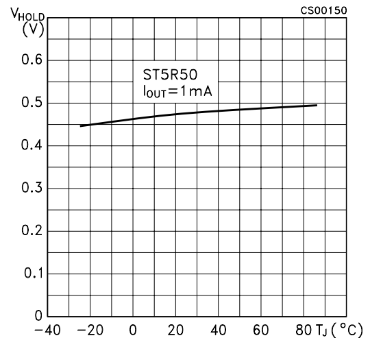
Figure 29: Hold-on Voltage vs Temperature
