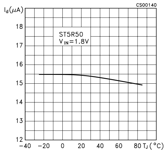
Figure 31: No Load Input Current vs Temperature
