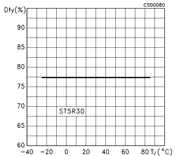
Figure 17: Oscillator Duty Cycle (@ MAX Freq.) vs Temperature
