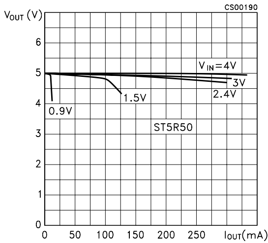
Figure 7: Output Voltage vs Output Current
