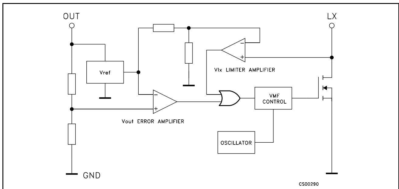
Figure 1: Schematic Diagram
