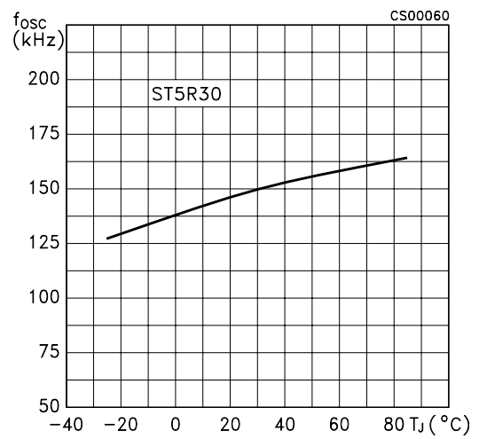
Figure 15: Maximum Oscillator Frequency vs Temperature
