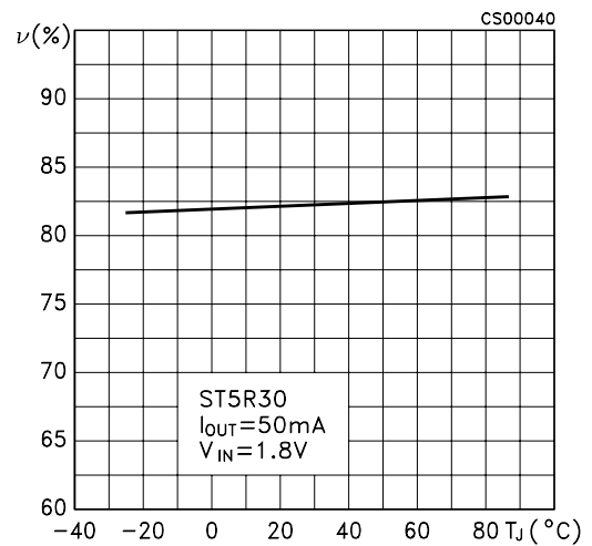
Figure 11: Efficiency vs Temperature
