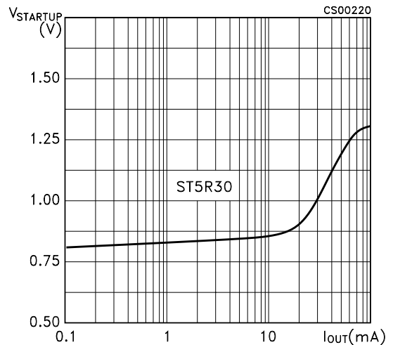
Figure 23: Start-up Voltage ( V_{IN} - V_F ) vs Output Current
