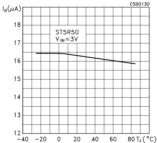
Figure 30: No Load Input Current vs Temperature
