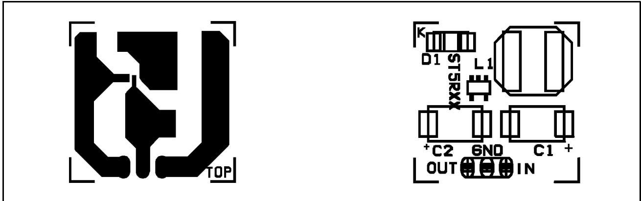
Figure 5: Typical Demoboard
