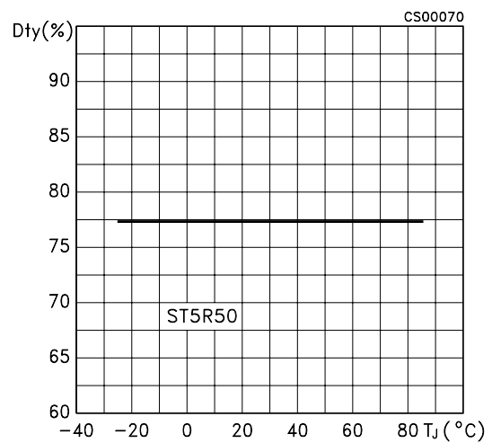
Figure 16: Oscillator Duty Cycle (@ MAX Freq.) vs Temperature
