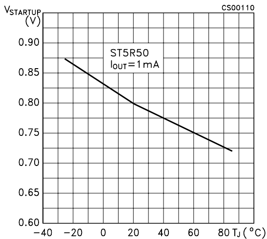
Figure 20: Start-up Voltage ( V_{IN} - V_F ) vs Temperature
