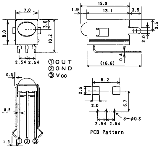
NJL64H000A UNIT : mm
