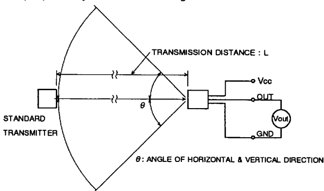
Fig. 3 TEST SYSTEM
