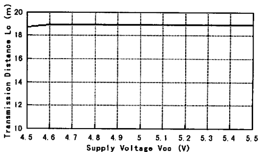
Transmission Distance vs. Supply Voltage ( T_a=25^\circ\text{C} )
