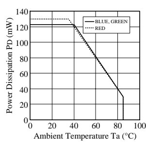
■ Ambient Temperature vs. Power Dissipation *
