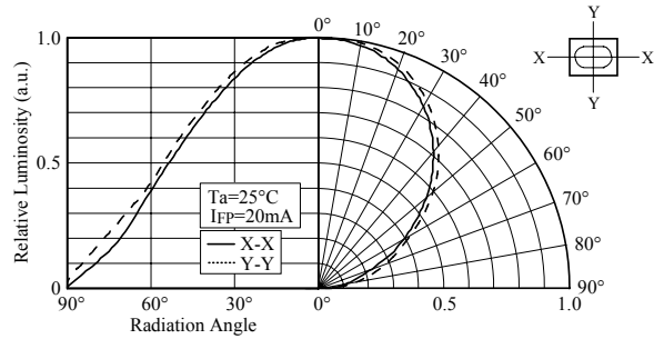
■ Directivity
