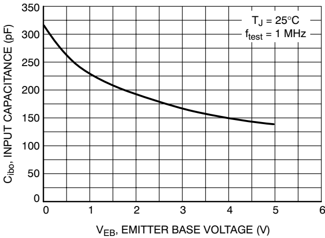
Figure 10. Input Capacitance
