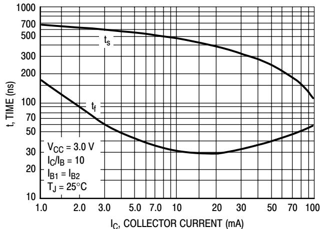
Figure 14. Turn-Off Time
