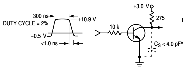
Figure 1. Turn–On Time
