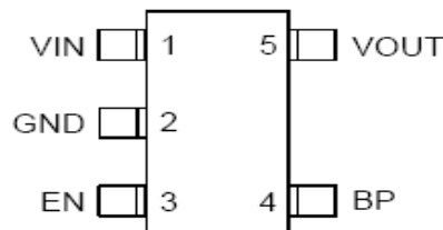
SOT23-5(Top View)
