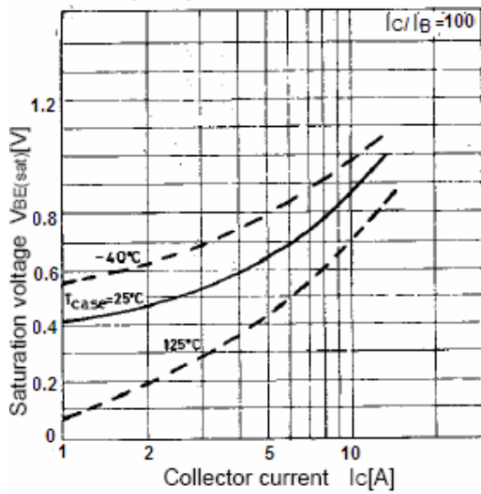
V_{BE(sat)}-I_C Characteristics
