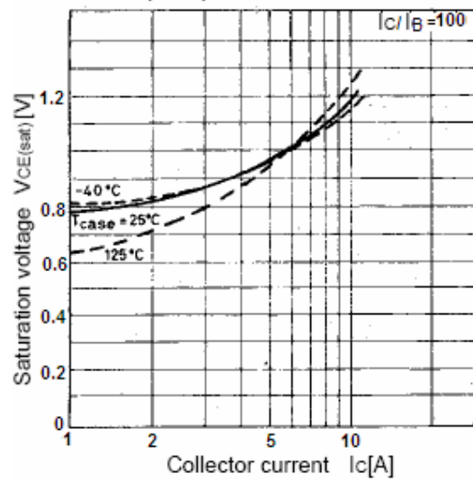
V_{CE(sat)}-I_C Characteristics
