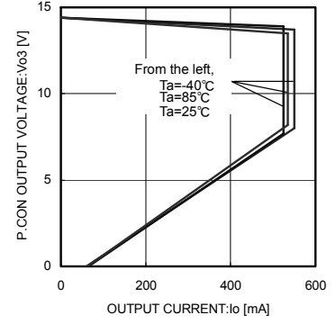
Fig. 13 P.CON Load Regulation
