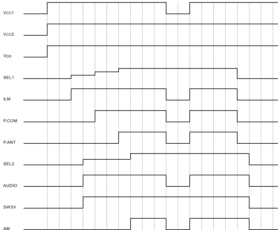
Fig.44 Timing Chart
