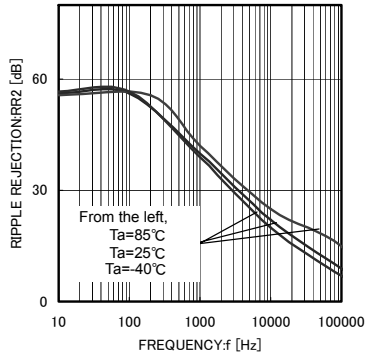
Fig. 11 AUDIO Ripple Rejection Ratio ( I_o = 200 \text{ mA} )
