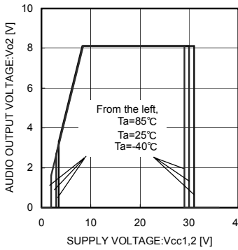
Fig.36 Overvoltage Operation
