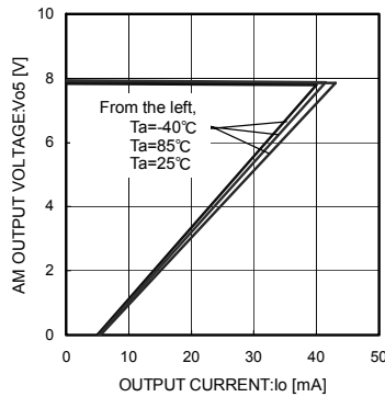
Fig. 18 AM Load Regulation
