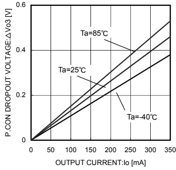
Fig. 14 P.CON Dropout Voltage
