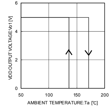
Fig.37 Thermal Shutdown Operation
