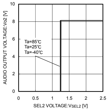
Fig.32 AUDIO Input Threshold Voltage
