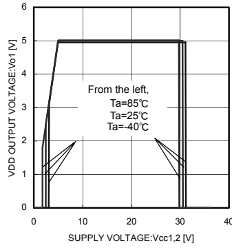
Fig.3 VDD Line Regulation ( I_o = \text{No load} )
