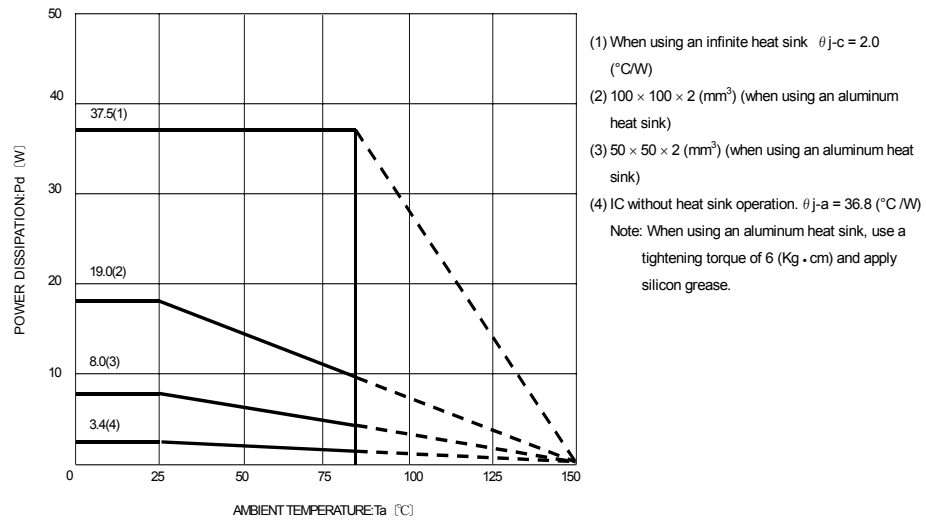
Fig.46 Power Dissipation Characteristics
