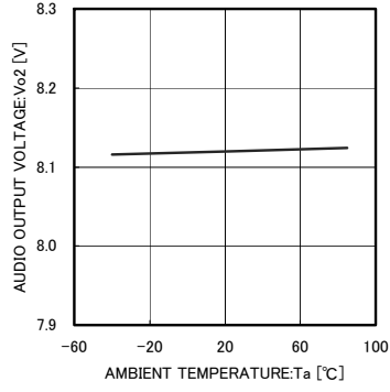
Fig. 12 AUDIO Output Voltage vs Temperature
