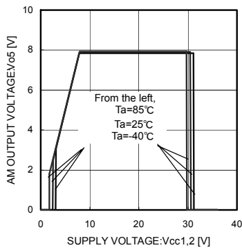
Fig. 17 AM Line Regulation ( I_o = \text{No load} )
