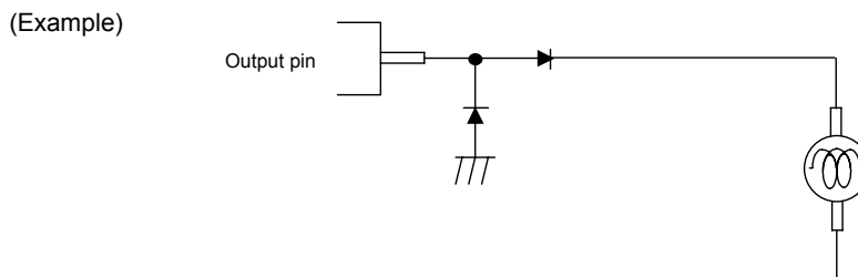
Fig.51 Example of Protective Diode Insertion
