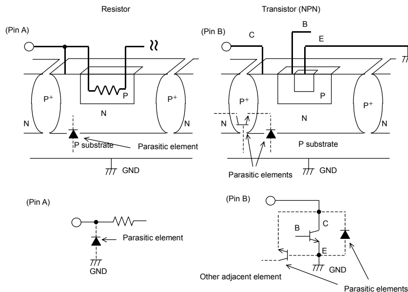
Fig.48 Example of a Simple Monolithic IC Architecture
