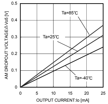
Fig. 19 AM Dropout Voltage ( V_{cc1} = V_{cc2} = 7.5 \text{ V} )
