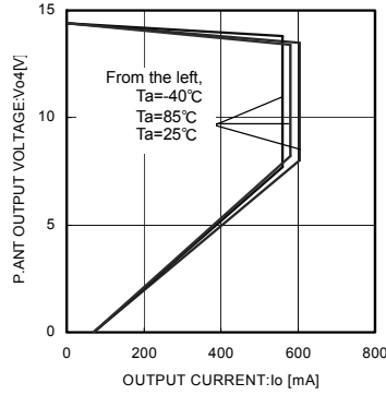
Fig. 15 P.ANT Load Regulation
