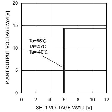
Fig.31 P.ANT Input Threshold Voltage
