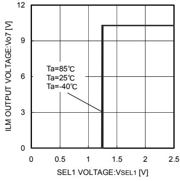
Fig.29 ILM Input Threshold Voltage
