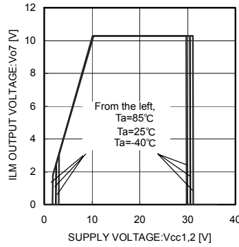
Fig.24 ILM Line Regulation (Io = No load)
