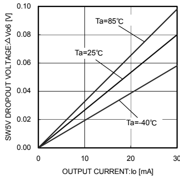
Fig.23 SW5V Dropout Voltage (Vcc1 = Vcc2 = 10 V)
