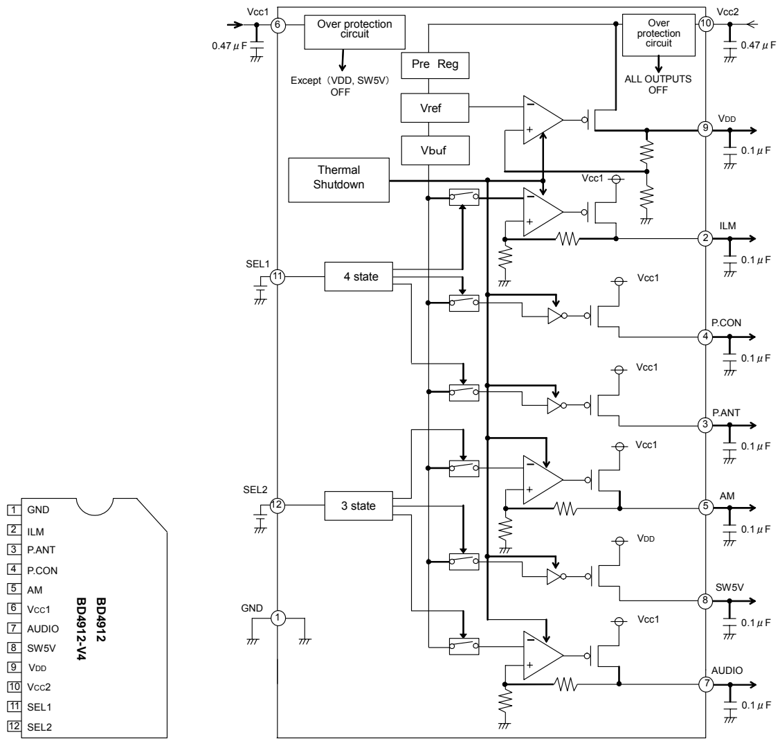
Fig.38 Pin Assignment Diagram
