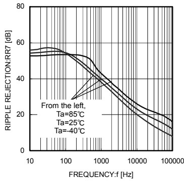
Fig.27 ILM Ripple Rejection Ratio (Io = 200 mA)
