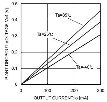
Fig. 16 P.ANT Dropout Voltage
