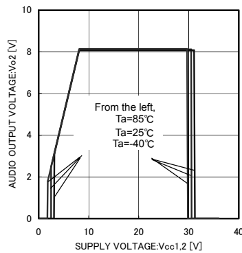
Fig.8 AUDIO Line Regulation ( I_o = \text{No load} )
