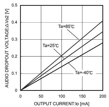
Fig.10 AUDIO Dropout Voltage ( V_{CC1} = V_{CC2} = 7.8 \text{ V} )
