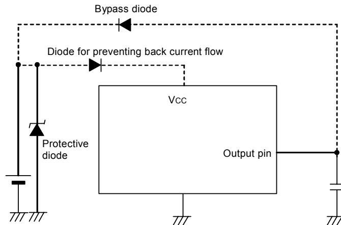
Fig.49 Example of Bypass Diode Insertion to Prevent Back Current Flow
