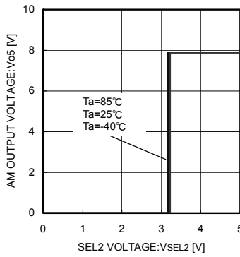
Fig.33 AM Input Threshold Voltage
