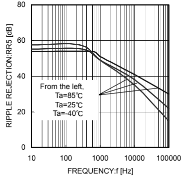
Fig.20 AM Ripple Rejection Ratio (Io = 25 mA)
