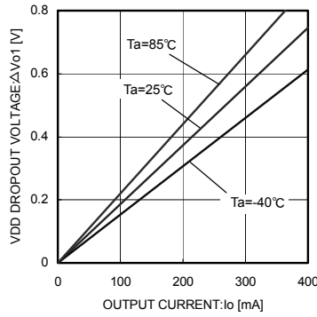
Fig.5 VDD Dropout Voltage ( V_{CC1} = V_{CC2} = 4.8 \text{ V} )
