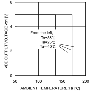
Fig.4 VDD Load Regulation
