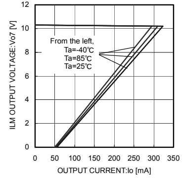
Fig.25 ILM Load Regulation
