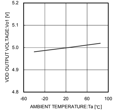
Fig.7 VDD Output Voltage vs Temperature
