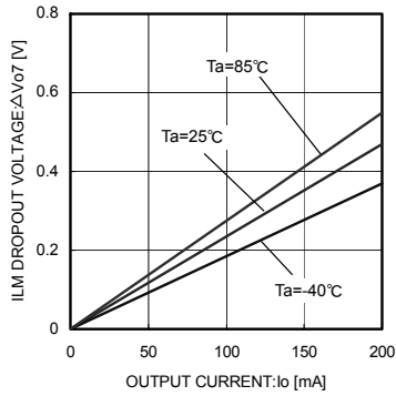
Fig.26 ILM Dropout Voltage (Vcc1 = Vcc2 = 9.9 V)
