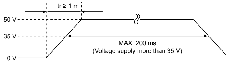
Fig.1 Peak Supply Voltage Waveform
