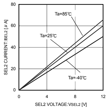
Fig.35 SEL2 Input Current
