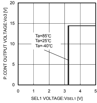
Fig.30 P.CON Input Threshold Voltage
