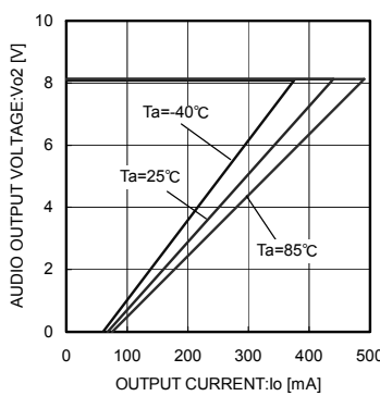
Fig.9 AUDIO Load Regulation
