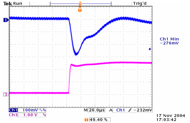
Figure 24: Typical transient response to step load change at 2.5A/μs from 50% to 100% of I_o , max at 3.3Vin, 2.5V out (Cout = ceramic, 10μF tantalum)
