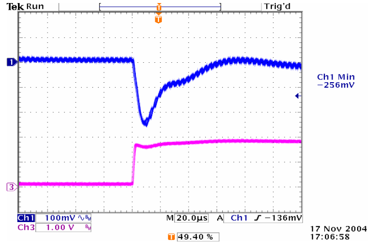
Figure 26: Typical transient response to step load change at 2.5A/μs from 50% to 100% of I_o , max at 3.3Vin, 1.8V out (Cout = ceramic, 10μF tantalum)
