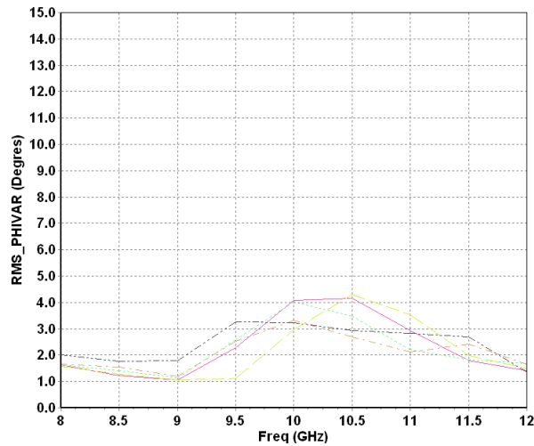
RMS phase variation in RX mode Tuning attenuator state 1 Phase shifter states 0-8-16-32-63
