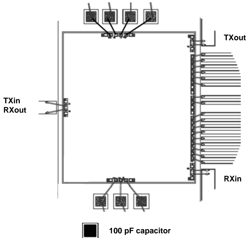
Assembly diagram
