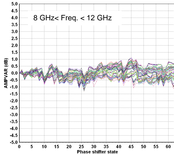
Amplitude variation vs. phase state in RX and TX mode Tuning attenuator state 1 Fine attenuator states 0-8-16-32
