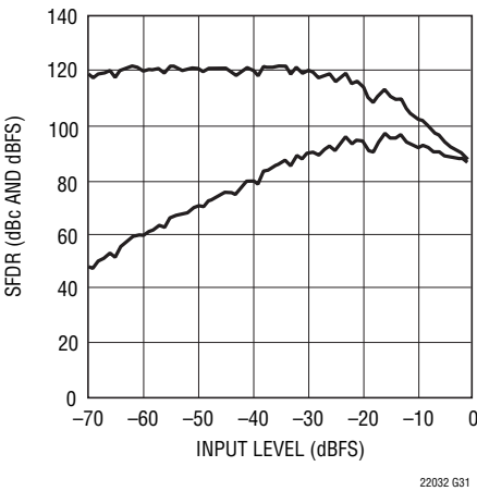
LTC2203: SFDR vs Input Level, f_{IN} = 70.1\text{MHz} , \text{PGA} = 0 , Dither "On"
