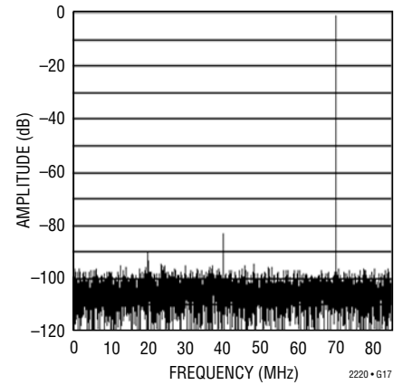
LTC2220: 8192 Point FFT, f_{IN} = 70\text{MHz} , -1dB, 2V Range, LVDS Mode
