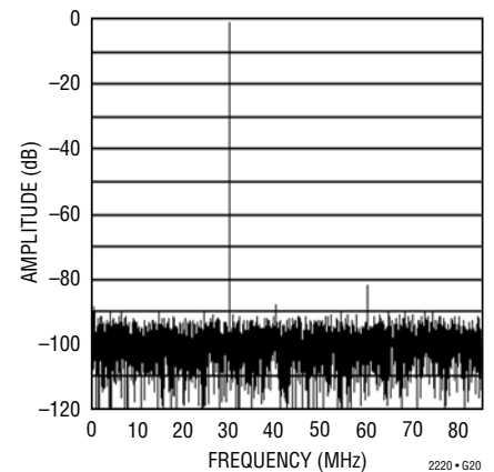
LTC2220: 8192 Point FFT, f_{IN} = 140\text{MHz} , -1dB, 1V Range, LVDS Mode
