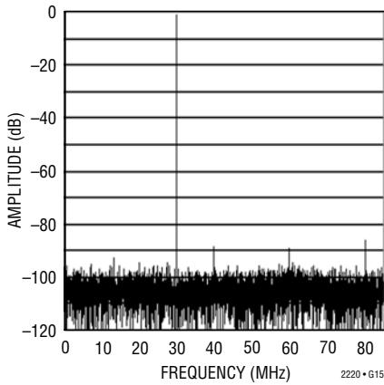
LTC2220: 8192 Point FFT, f_{IN} = 30\text{MHz} , -1dB, 2V Range, LVDS Mode
