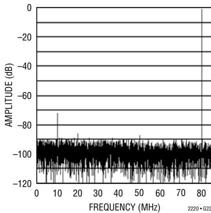
LTC2220: 8192 Point FFT, f_{IN} = 250\text{MHz} , -1dB, 1V Range, LVDS Mode
