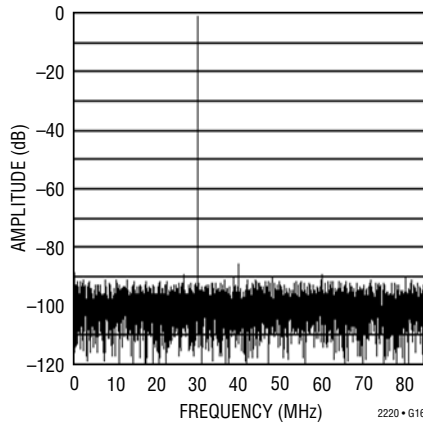
LTC2220: 8192 Point FFT, f_{IN} = 30\text{MHz} , -1dB, 1V Range, LVDS Mode
