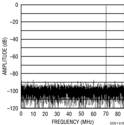
LTC2220: 8192 Point FFT, f_{IN} = 70\text{MHz} , -1dB, 1V Range, LVDS Mode
