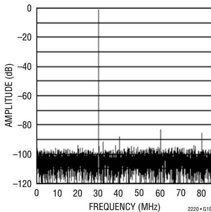
LTC2220: 8192 Point FFT, f_{IN} = 140\text{MHz} , -1dB, 2V Range, LVDS Mode
