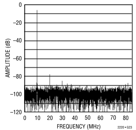
LTC2220: 8192 Point FFT, f_{IN} = 500\text{MHz} , -6dB, 1V Range, LVDS Mode
