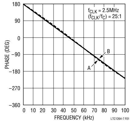
Figure 1. Phase Response in the Passband (Note 2)
