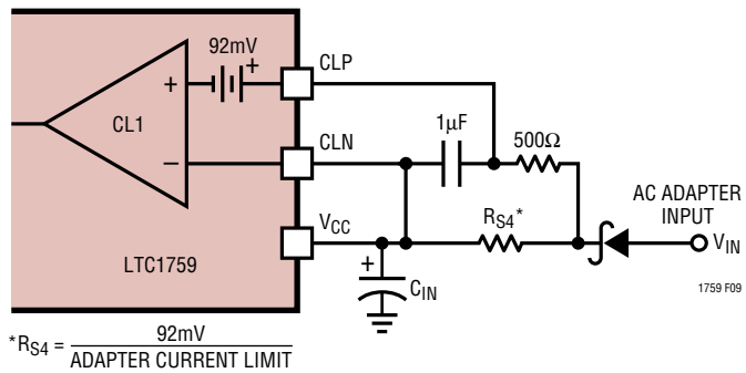
Figure 9. Adapter Current Limiting
