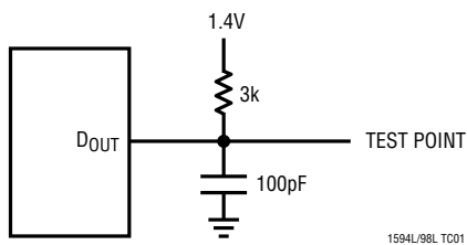
Load Circuit for t_{DQ} , t_r and t_f
