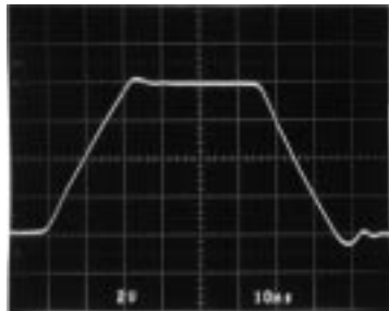
V_S = \pm 5V A_V = +1 R_L = 1k 10ns/DIV 1809 G40
