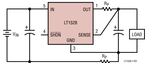
Figure 1. Kelvin Sense Connection
