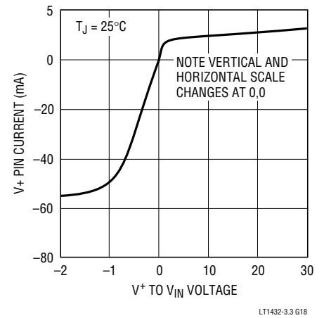
Start-up Switch Characteristics
