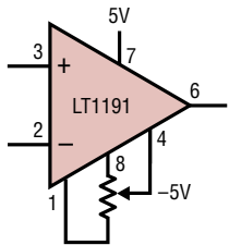
INPUT OFFSET VOLTAGE CAN BE ADJUSTED OVER A ±100mV RANGE WITH A 1kΩ TO 10kΩ POTENTIOMETER
