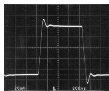
Small-Signal Response
