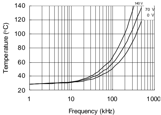
Figure 26. IRS2304 vs. Frequency (IRFPE50), R_{gate} = 10 \Omega, V_{cc} = 15 V
