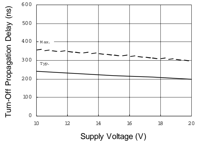
Figure 5B. Turn-Off Propagation Delay vs. Supply Voltage
