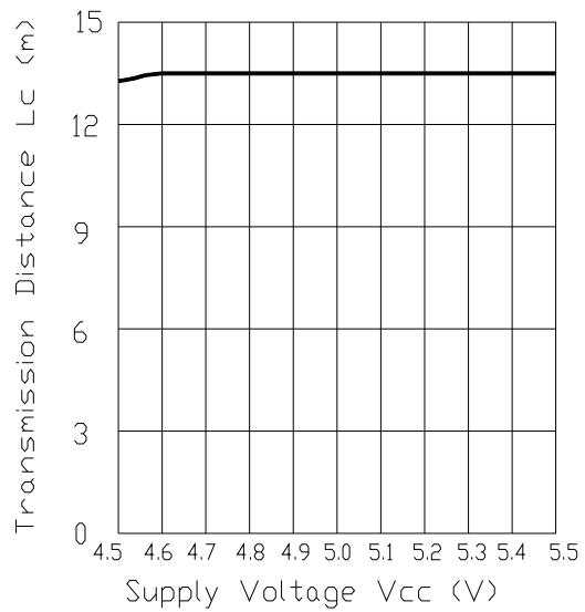
Fig.-7 Arrival Distance vs. Supply Voltage
