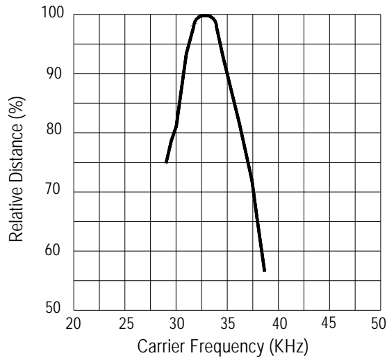
Fig.-8 Relative Transmission Distance Center Carrier Frequency
