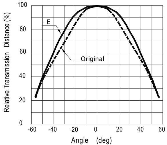
Fig.-5 Relative Transmission Distance vs. Direction
