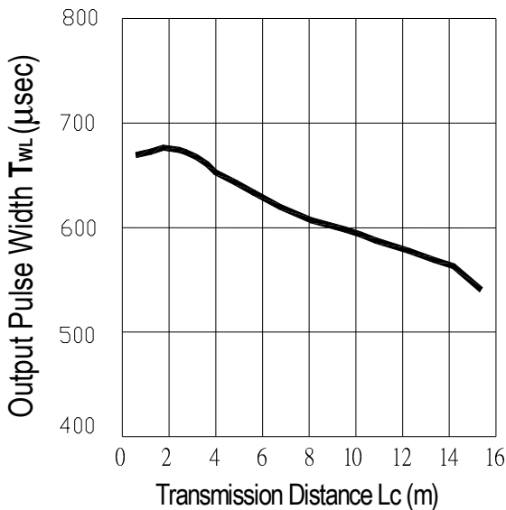
Fig.-6 Output Pulse Length vs. Arrival Distance
