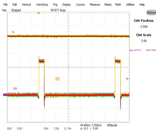
Fig. 18: Inductor node at 8A, sourcing current, Ch 3 :SW, Ch 4 :I out
